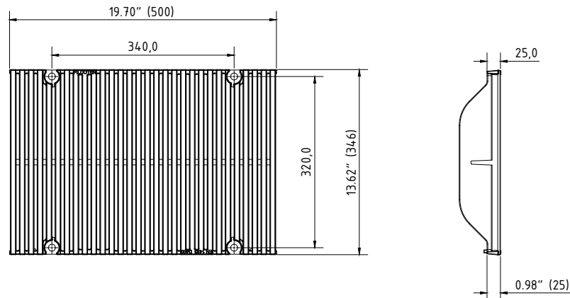
D400kN SW5.7mm: GJS 17030183
