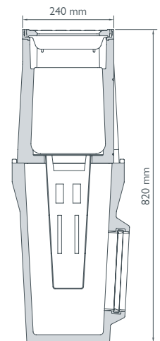
Sump unit, two-piece
