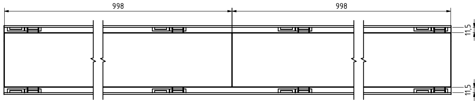
Variante A / variant A Steinhöhe 20mm / slab height 20mm ( 1 : 2 )
