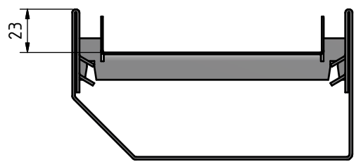
Variante A / variant A Steinhöhe 20mm / slab height 20mm ( 1 : 2 )
