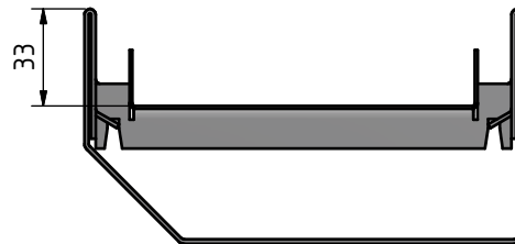
Variante B / variant B Steinhöhe 30mm / slab height 30mm ( 1 : 2 )
