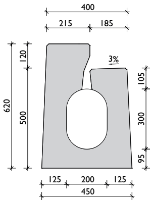
Profil I-5 Bordstein links
