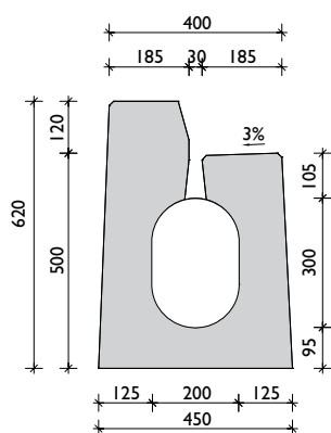
Profil I-3 Bordstein links
